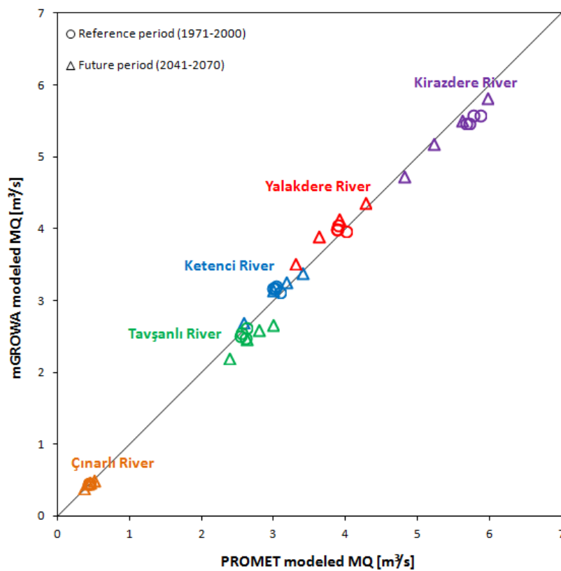
Fig 10. PROMET and mGROWA modeled mean streamflow in [m^3/s] of the 5 major rivers in Izmit Bay for the reference period (1971-2000) and the future period (2041-2070). Displayed are the MQs of all four used climate model inputs
