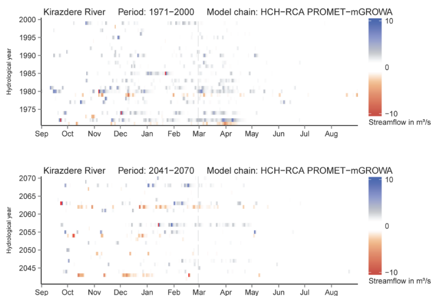
Fig 14. Differences in the raster hydrographs for the Kirazdere River (HCH-RCA PROMET-mGROWA)
